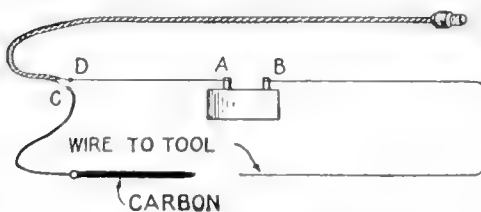
Connections to a rheostat and carbon for writing letters on steel
